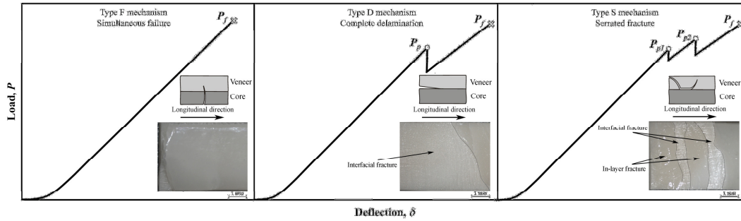
Figure 1: Failure mechanisms of the two layered zirconia-veneer specimens together with schematic depictions of the force-deflections curves and optical observations of the fracture surfaces.
